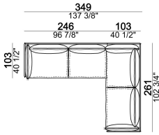
Composition "C" (left unit 246x103 cm + left corner sofa 261x103 cm)
